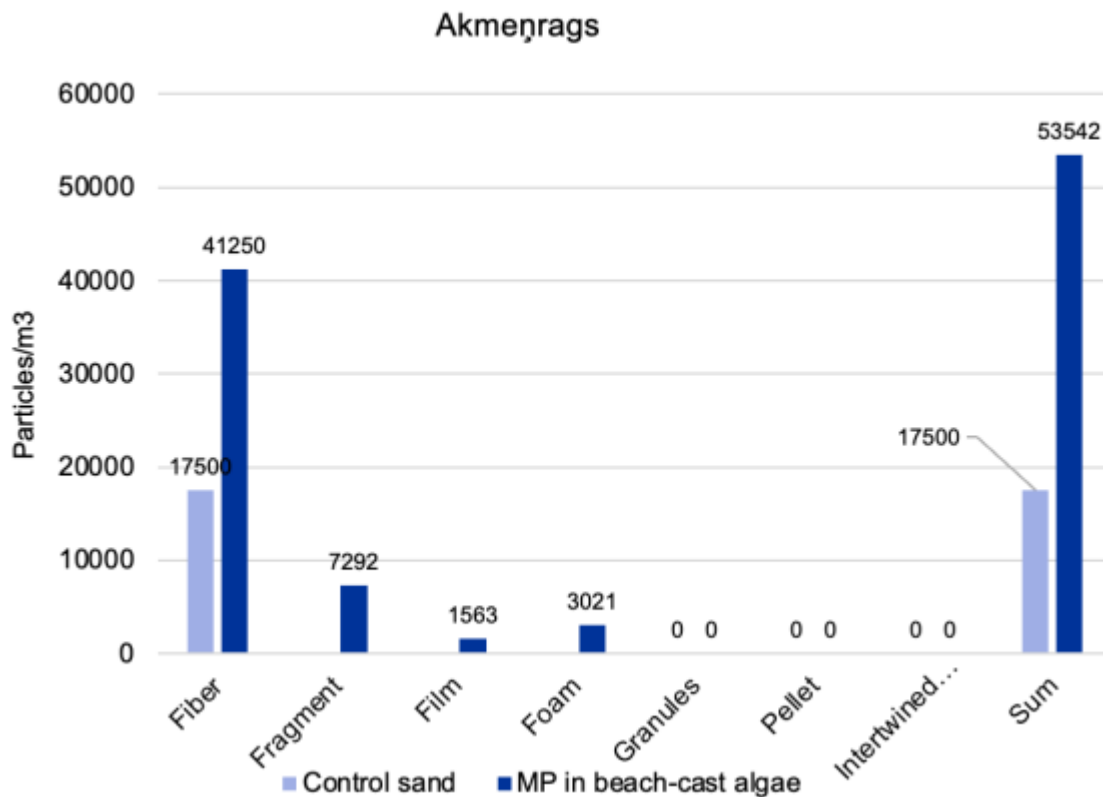
Fig.3 Types of microplastic particles and their abundance in the beach wrack (beach-cast algae) per m 3 near Akmeņrags, Latvia in 2021.
